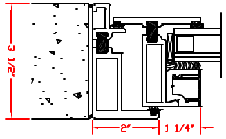
2 SILL DETAIL 3 SCALE : NTS
