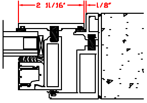
2 HEAD DETAIL 1 SCALE : NTS
